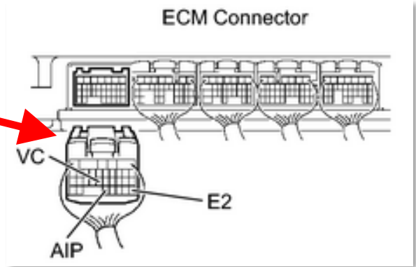
Figure 14 – Pressure Sensor Wires to Tap into.
