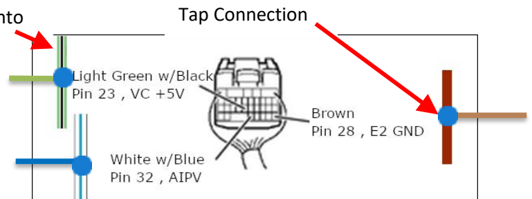
Figure 21 - GX470 Wire Colors (shown in Figure 19).
