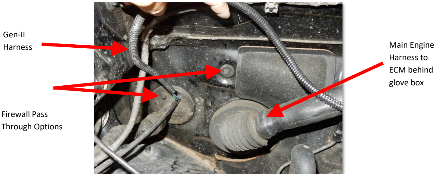
Figure 10 - Route End of Harness Through the Firewall for ECM Connections.
