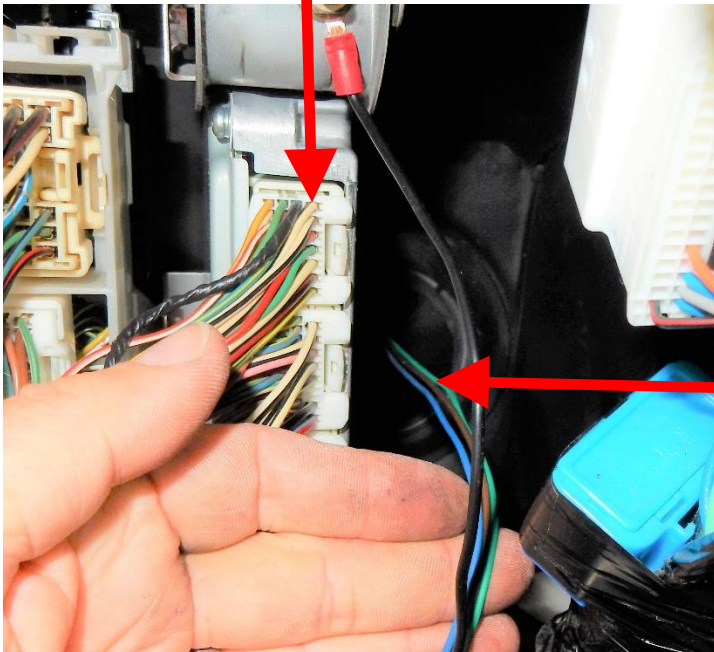
Figure 15 - Gen-II Harness Wires.
